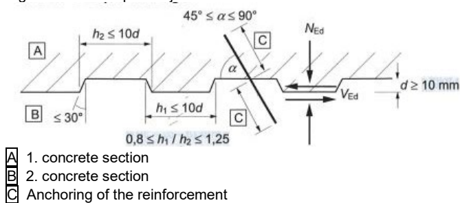
Figure 6.8 - Examples of joints
