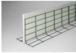
Stremaform® ekspansionsfuge
