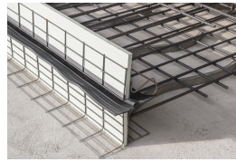
Formwork elements for expansion joints Stremaform® with rubber water bar cage
