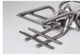
Shear force dowel Egcodorn®
