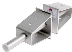
Shear force dowel Egcodorm® DND
